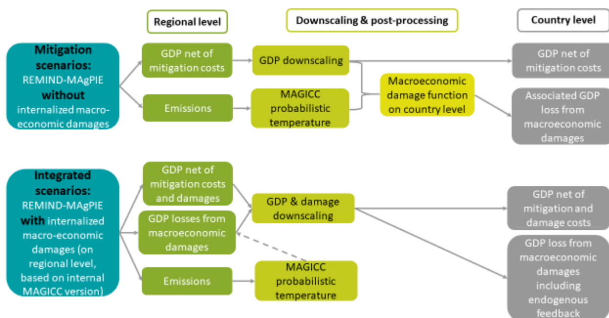
Figure 71. Non-Integrated REMIND runs vs Integrated REMIND runs
